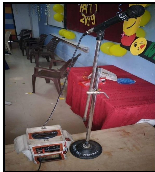
Amplifier with speaker (Battery backup & Charging)
